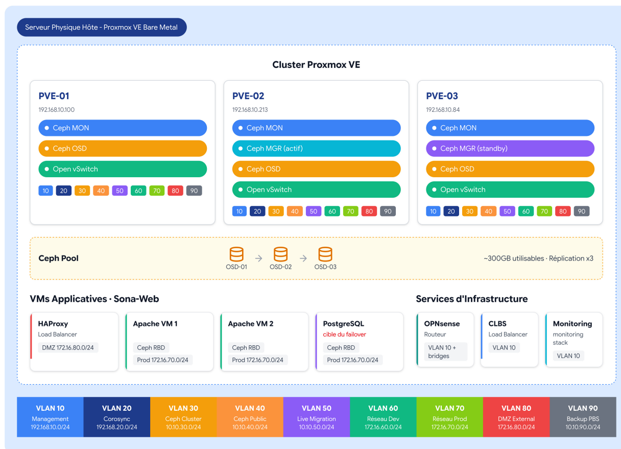
FIGURE III.1 – Architecture Globale de l'Infrastructure HCI
